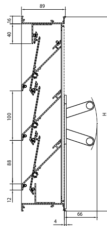
Without flange ref. 427ZF
