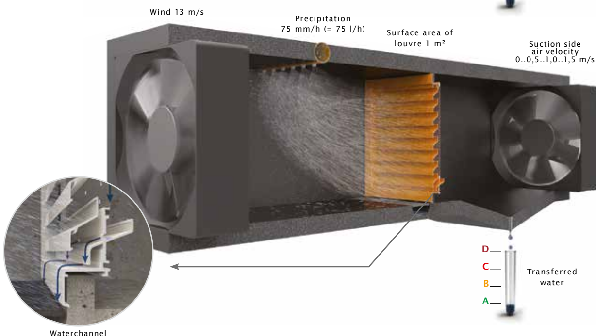
With waterchannel Test on a type 411 louvre with waterchannel
