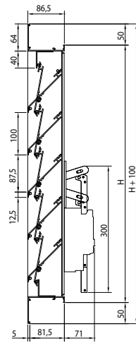
Type 427/4 220 V/24 V motor control Minimum louver height: 390 mm
