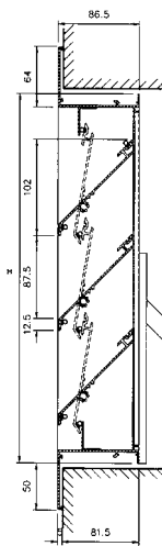
Type 427/1 Manual control Minimum louver height: 290 mm
